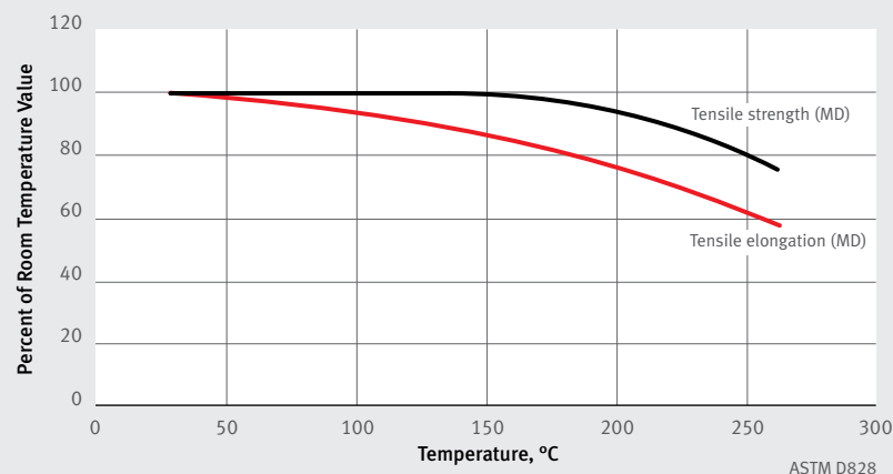
Figure 4. Temperature Effects on Mechanical Properties of DuPont® Nomex® 818 — 0.13 mm (5 mil)
