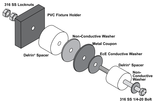
FIGURE 2. CONDUCTIVE WASHER
